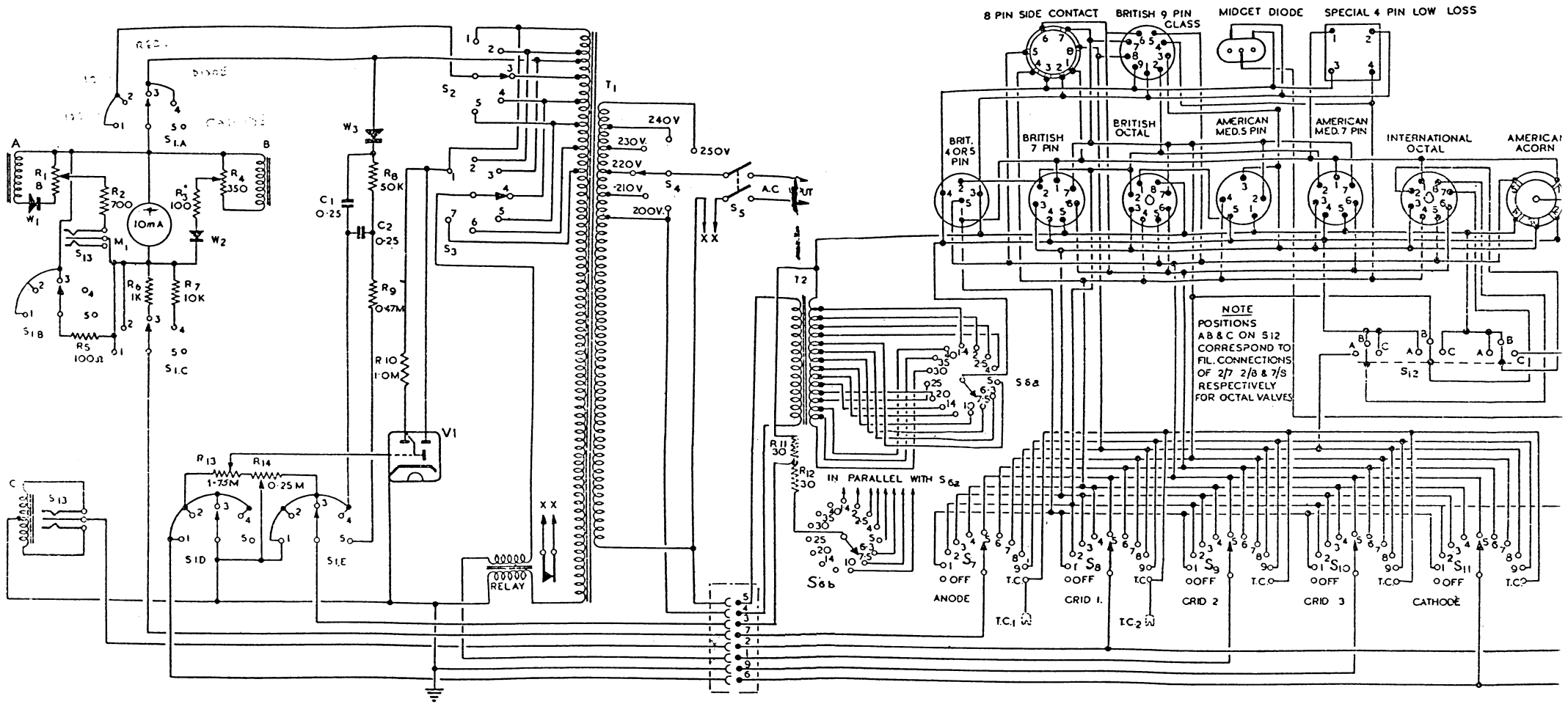
Fig. 4.—Valve tester, type 4A, circuit
